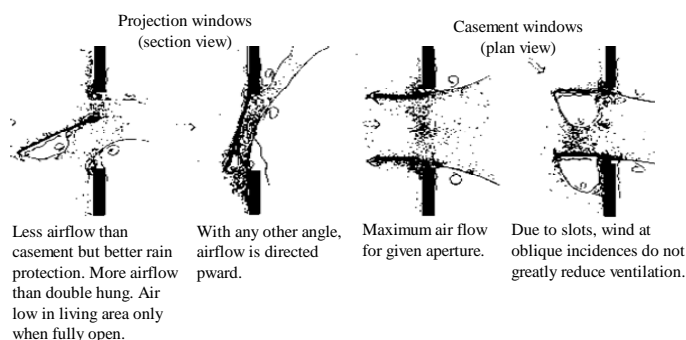
Fig. 1 Airflow patterns through windows
