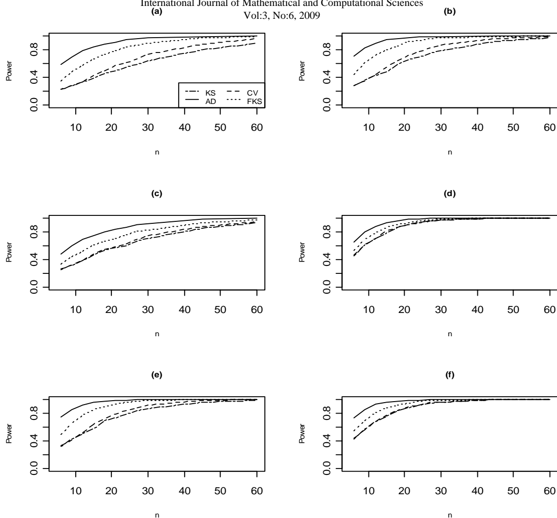
Fig. 2 Power comparison for normality test for various alternative hypotheses under RSS
