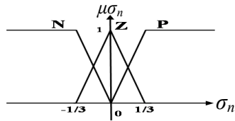
Fig. 3 The subordinate function of \sigma_n .
