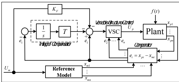
Fig. 2. The structure of FLSMFC system.
