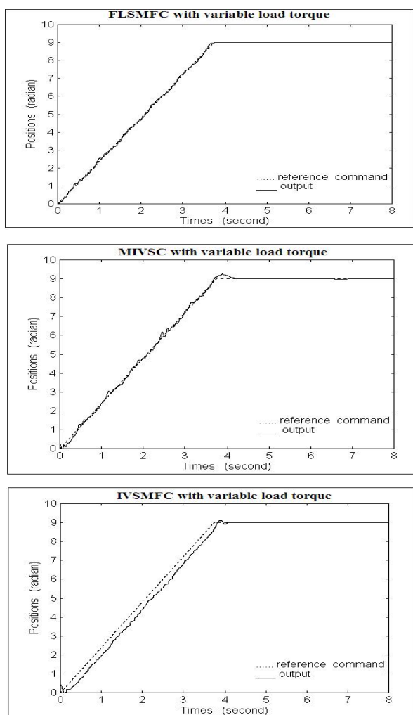
Fig. 9 Comparison of ramp position tracking.
