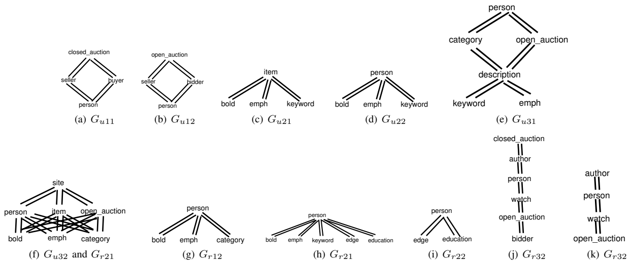
Fig. 4. Query Graphs
