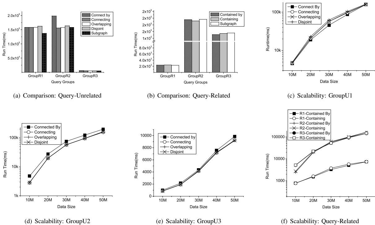
Fig. 5. Experimental Results
