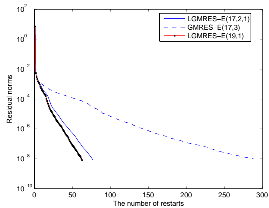
Fig. 5. The convergence curves of matrix memplus.
