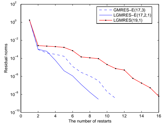
Fig. 4. The convergence curves of matrix wang4.
