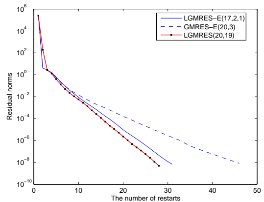
Fig. 6. The convergence curves of matrix orsreg1.
