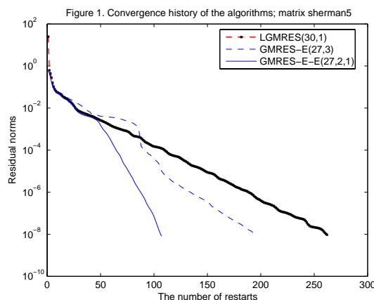
Fig. 1. The convergence curves of matrix sherman5.
