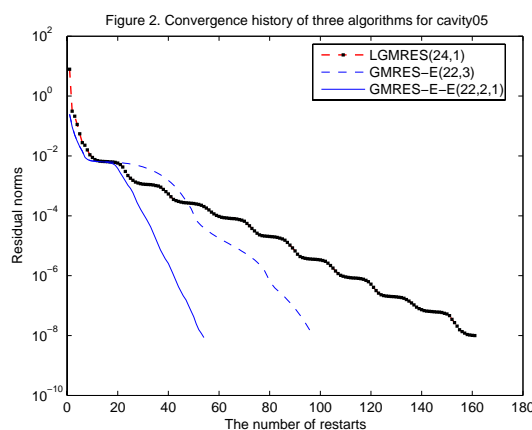
Fig. 2. The convergence curves of matrix cavity05.
