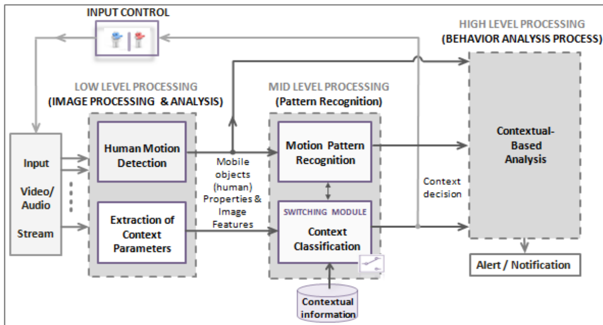
Fig. 1 Global ADABeV framework architecture
