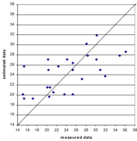
Fig. 5 Comparison of measured saturated hydraulic conductivity, K_s (m/day) and K_s estimated by equation (10)
