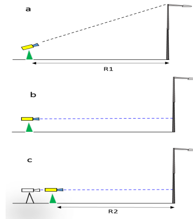
Fig. 5 Schematic of the three different setups of the test and picture of the light pole
