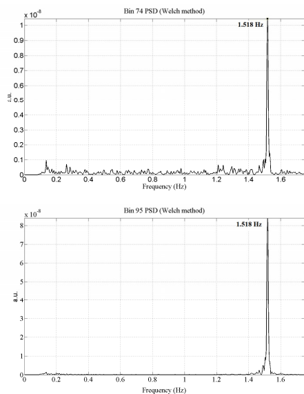
Fig. 9 PSD calculated for bin 74 and 95.
