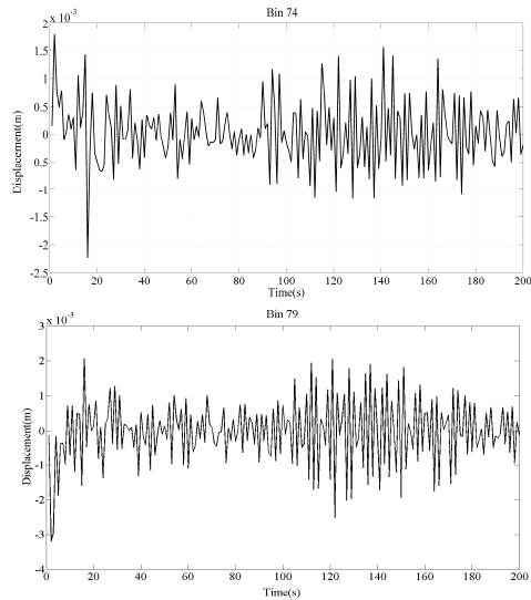
Fig. 8 Displacement samples corresponding to two different bins: 74 and 79.
